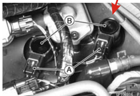
Ignition coils
