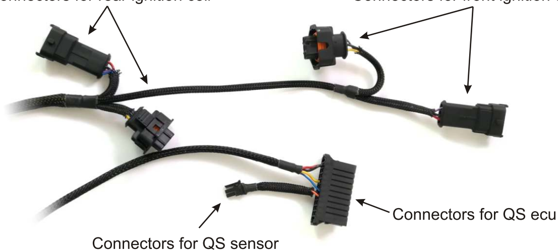
Connectors for rear ignition coil
