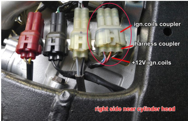
Pic.1 - location of 6way connector from Ignition coils
